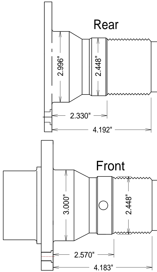
ERA GT Hub Dimensions
